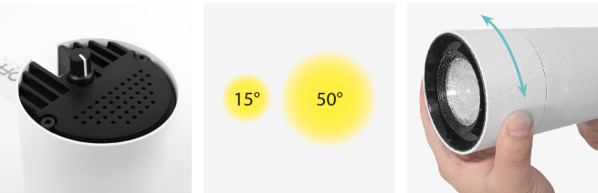
Potentiometer Adjustable beam angle Adjustable beam angle
